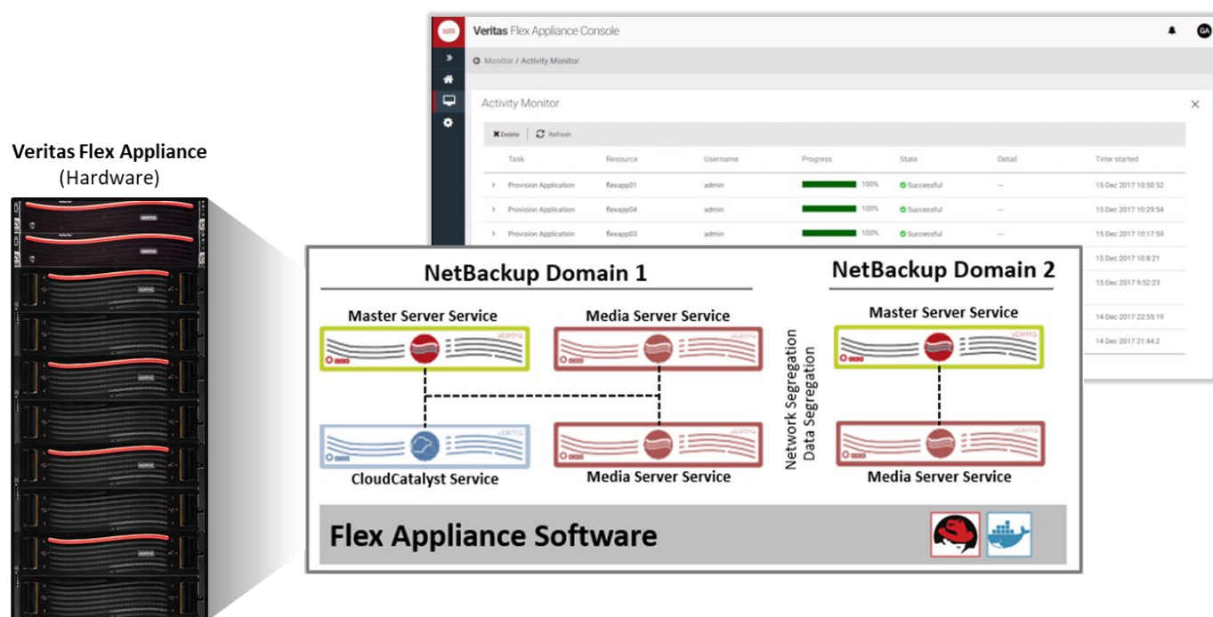
Figure 2. Solution Overview
