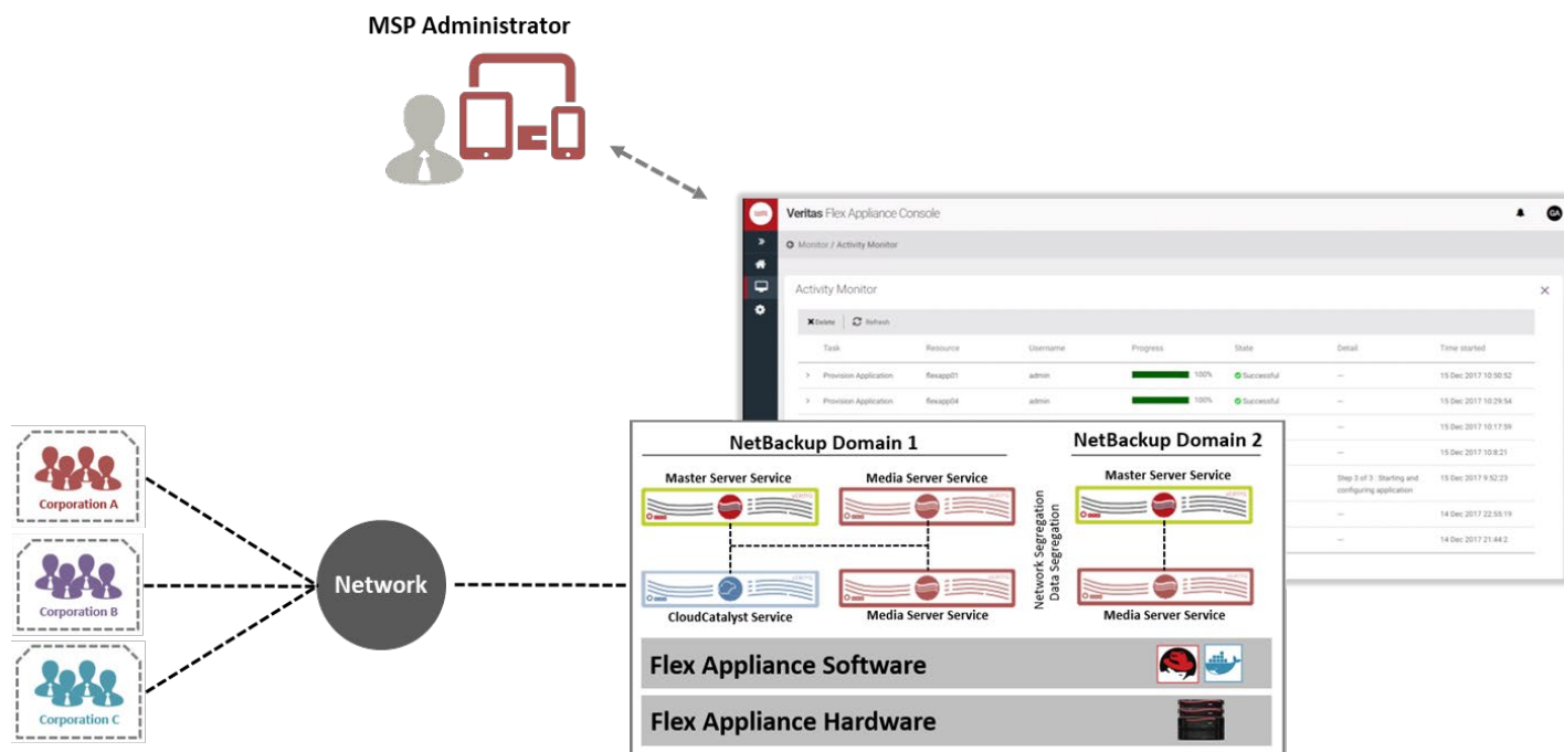
Figure 6. Multitenancy Overview
