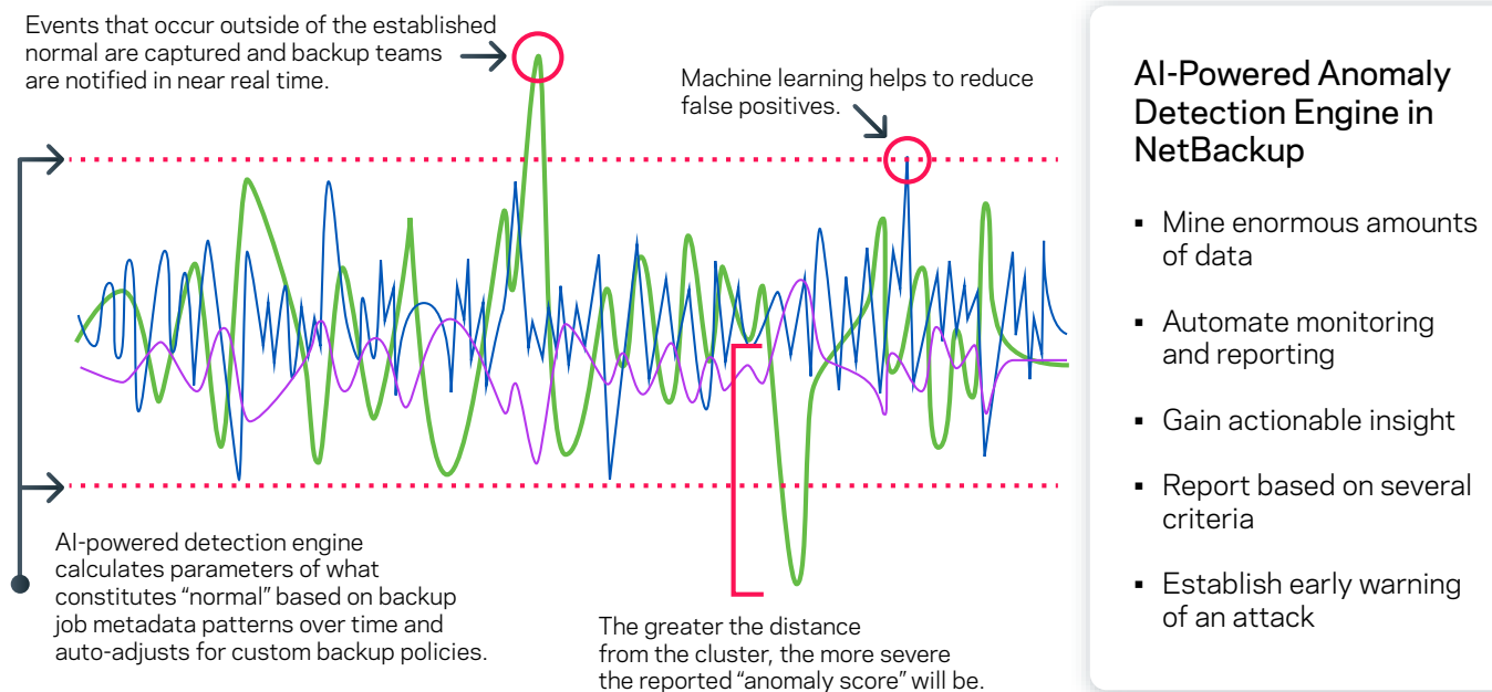
Figure 2. Understanding anomaly detection.
