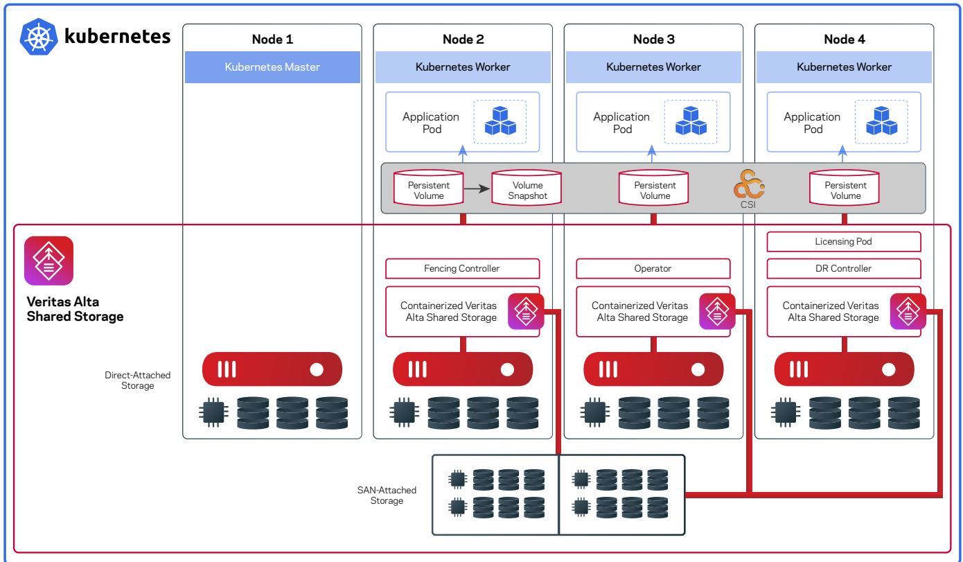
Figure 4. How Kubernetes and Veritas Alta Shared Storage integration provides high availability and persistent storage for containerized applications.
