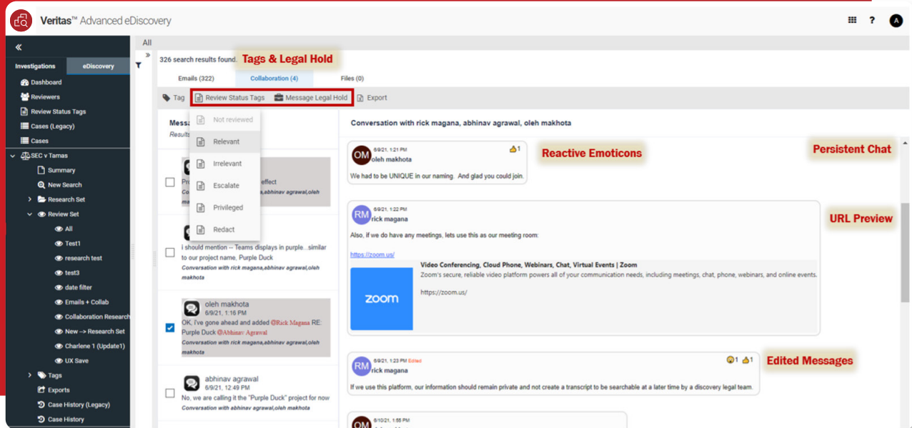
Figure 3. Collaboration View (MS Teams) with Tag & Legal Hold capabilities, and near-native chat review.
