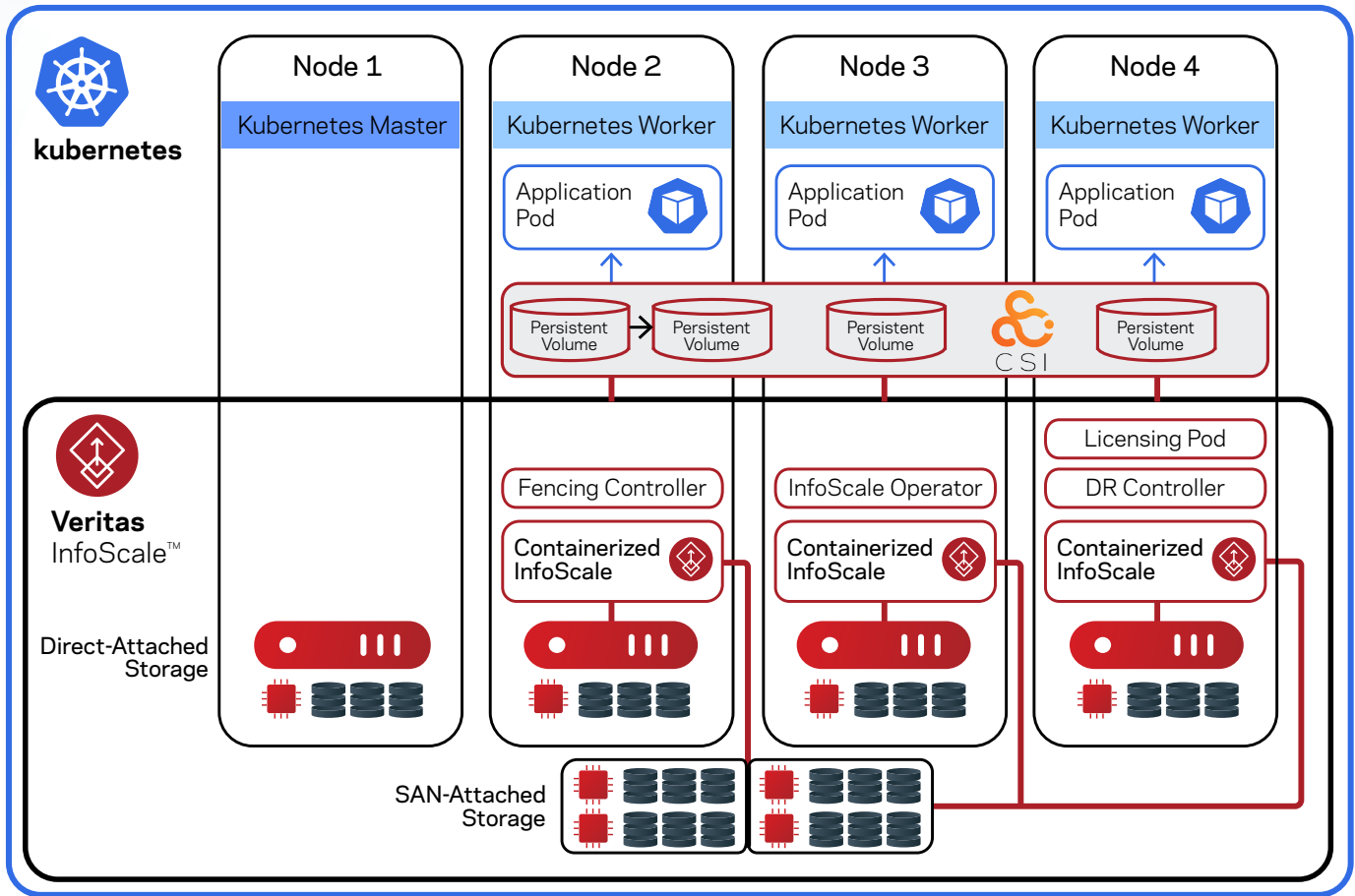
Figure 7. A Kubernetes cluster with InfoScale software-defined persistent storage.
