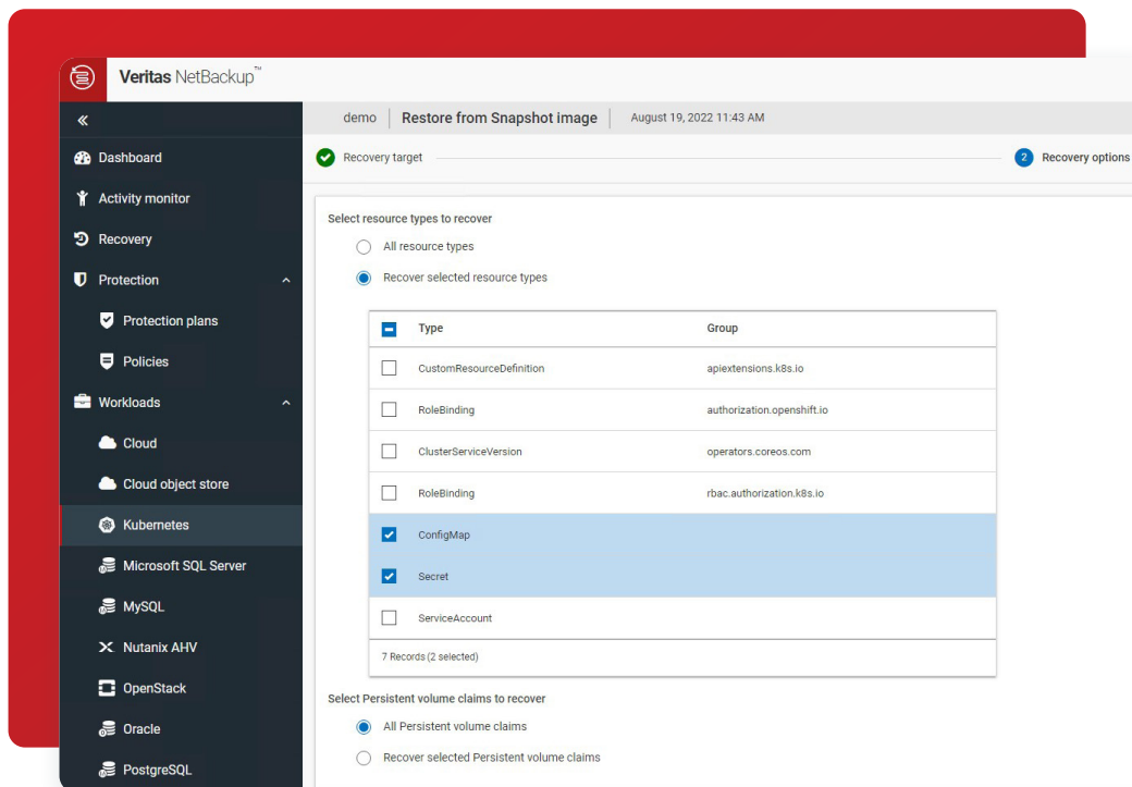
Figure 5. NetBackup for Kubernetes recovery options available from the management console.
