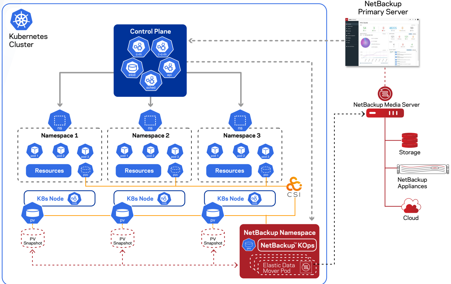
Figure 6. An overview of NetBackup data protection for Kubernetes clusters.
