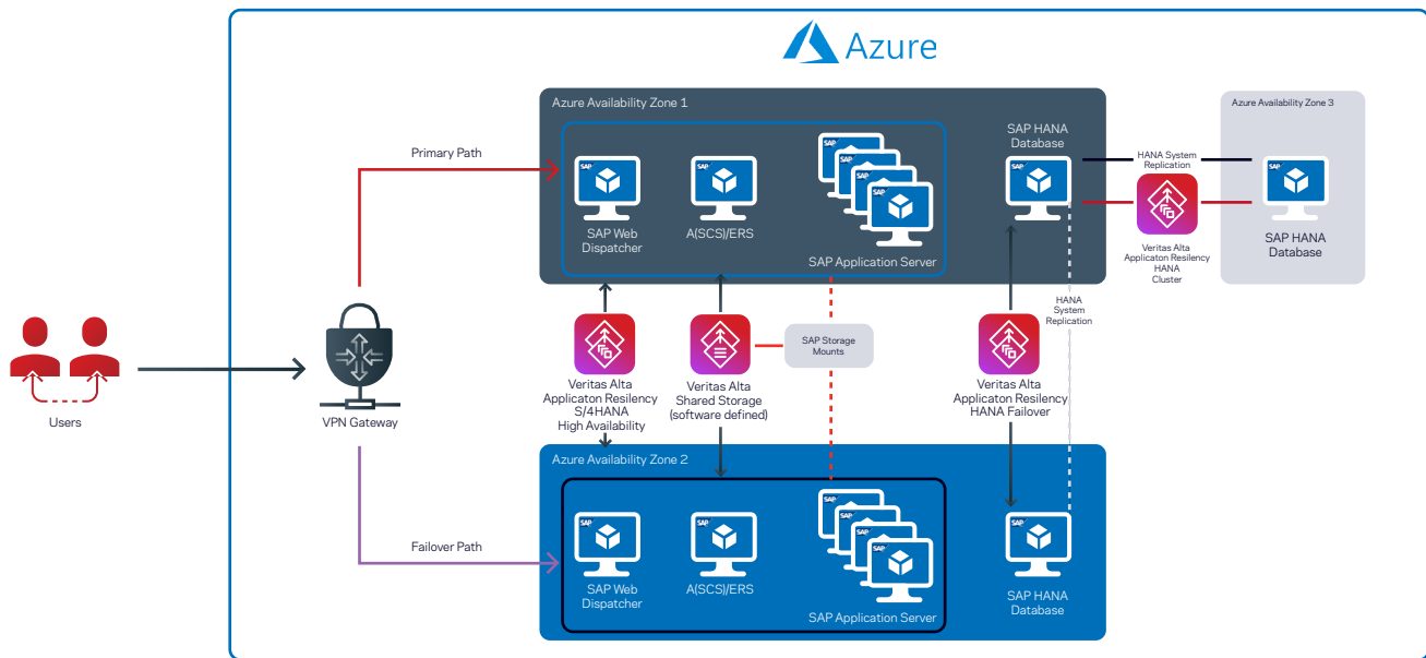
Figure 5. SAP S4/HANA with Veritas Alta Application Resiliency across Azure availability zones
