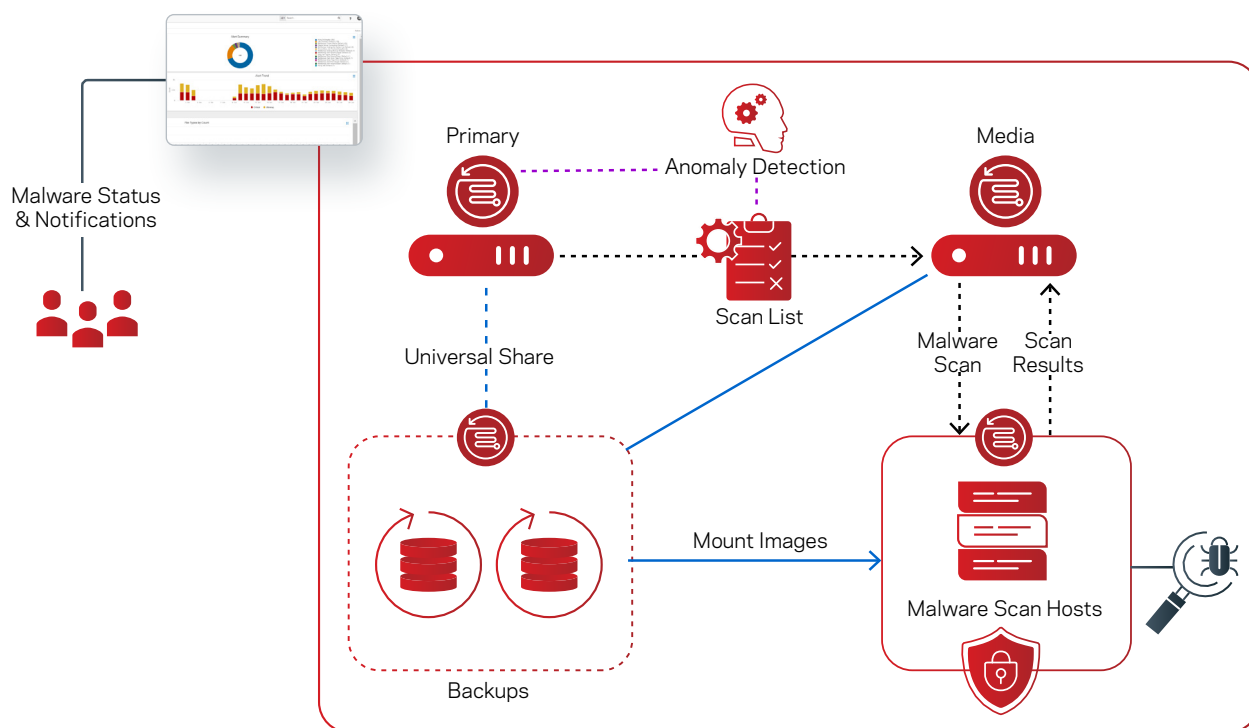
Figure 8. NetBackup integrated malware scanning
