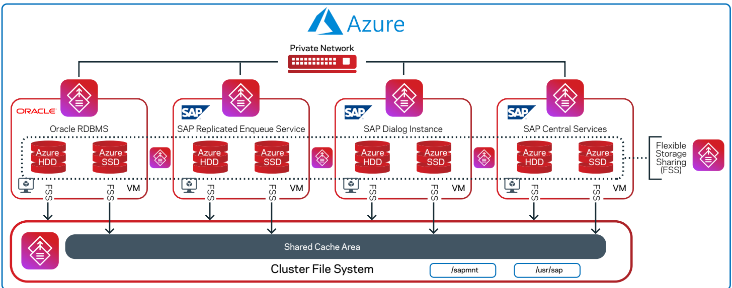
Figure 2. SAP S4/HANA running on Veritas Alta Shared Storage in Microsoft Azure
