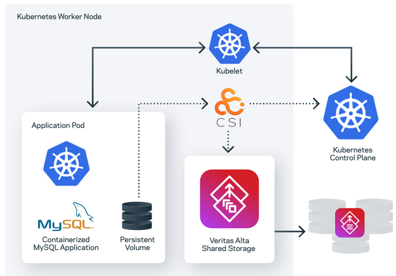
Figure 4. Veritas Alta Shared Storage CSI plug-in overview
