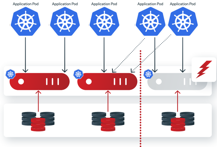
Figure 3. Veritas Alta Shared Storage I/O fencing in Kubernetes helps ensure data integrity
